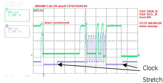
Example waveforms showing clock stretching.
