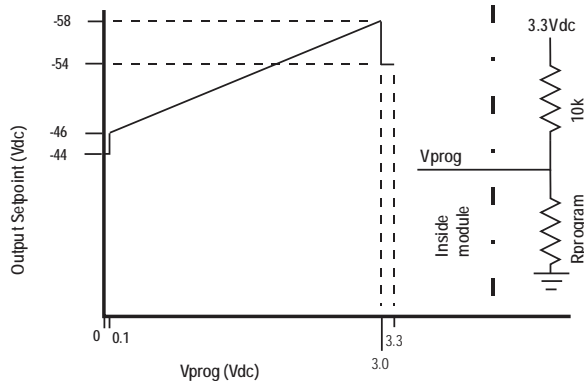
Factory default setting driven by Vprog
